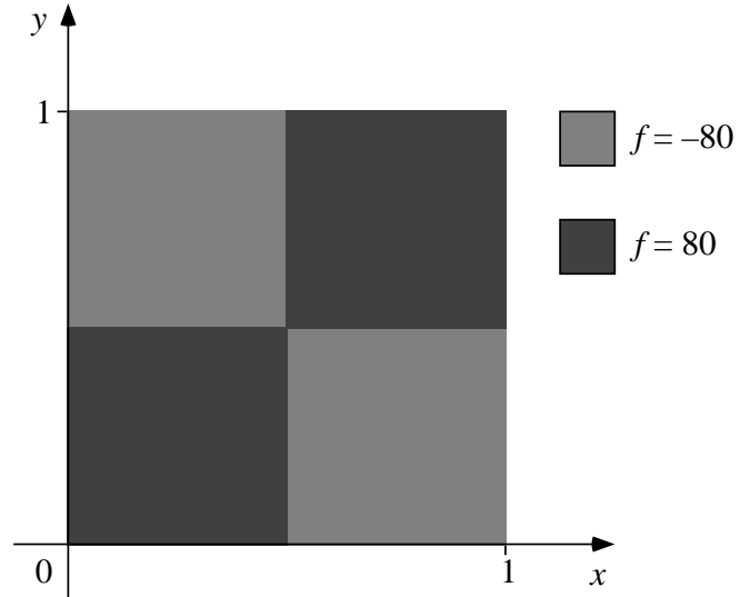
Figure 2. source term of problem 2
