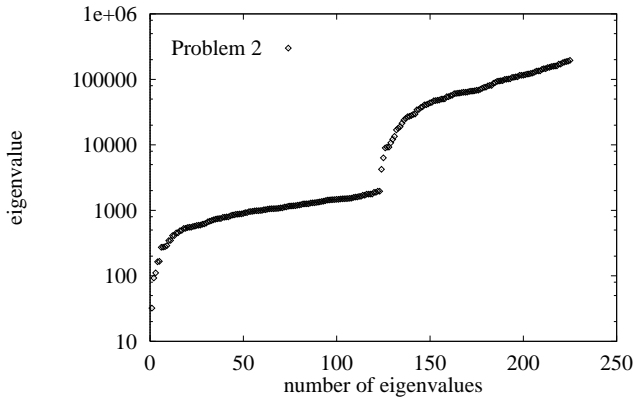
Figure 3. eigenvalues' distribution of a problem matrix
